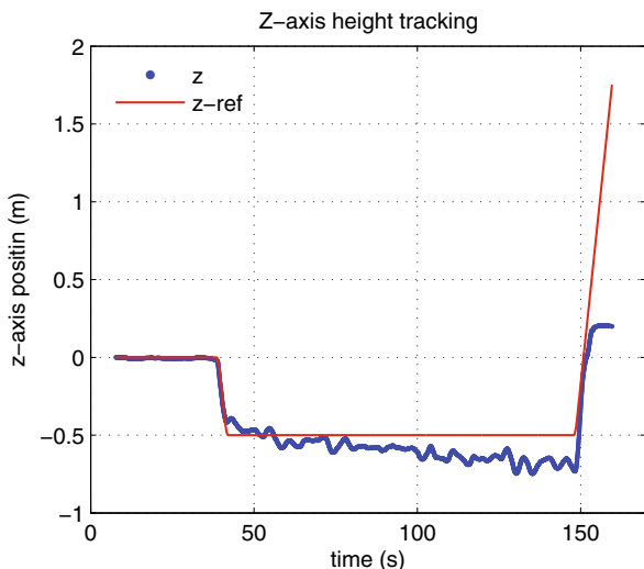
(c) z height tracking performance
