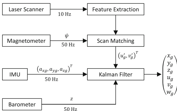
Fig. 7 The front-end state estimation diagram
