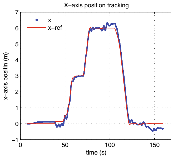
(a) x position tracking performance
