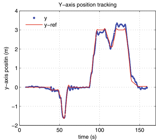
(b) y position tracking performance
